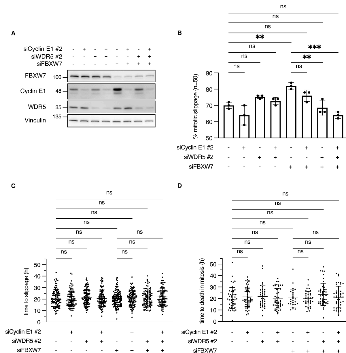
Figure 27: WDR5 depletion rescues the increase in chemoresistance after FBXW7 knockdown. A U2OS cells were transfected with siRNA targeting Cyclin E1, WDR5, FBXW7 or GI2, either alone or in combination, for 72 h. Cell lysates were analyzed by Western blotting. B 830 nM nocodazole were added to U2OS from A and mitotic cell fates were assessed by live-cell imaging. The time from mitotic entry to slippage C or cell death D was quantified for each analyzed cell. For each condition, n=50 cells were analyzed. *** p < 0.001, ** p < 0.01, * p < 0.05, ns p > 0.05, one-way ANOVA with Tukey post-hoc test, n=3. (Hänle-Kreidler et al. 2022).
